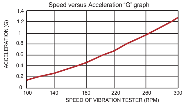
L.A.B. V-SERIES™ VIBRATION TESTER FIXED AT 1" DISPLACEMENT
